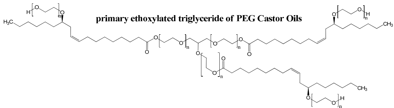
Figure 1. Glyceryl triricinoleyl polyethylene glycol
